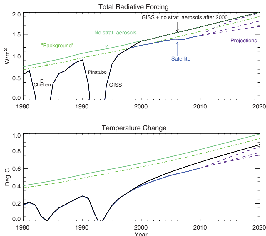
Fig. 4. Radiative forcing for six stratospheric aerosol forcing scenarios (top, also see Fig. 3) and the resulting change in global average temperature since preindustrial times as calculated by the Bern earth system model of intermediate complexity (bottom). Scenarios include: no stratospheric aerosol forcing (solid blue/green line); only background aerosol forcing with no volcanoes (dash-dotted green line); stratospheric aerosol forcing from GISS optical depths transitioning to no stratospheric aerosol forcing after 2000 (black line); forcing from GISS until 1998, then assuming forcing inferred from the global satellite optical depths (black followed by blue lines); this curve then splits into three future projections (dashed purple lines) as described for Fig. 3.
